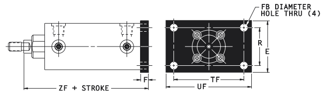
REAR FLANGE MOUNT (NFPA MF2)
