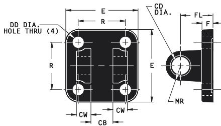
CLEVIS BRACKET
